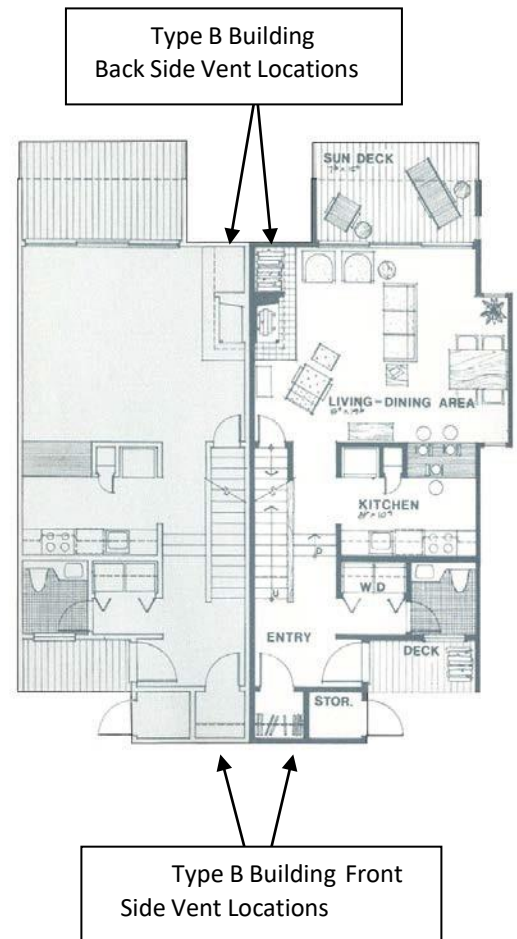
Figure 30. Type B building vent locations
